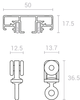
SLIM ROAD 01 Color: black, white Material: aluminum Compatible: textile, PVC
