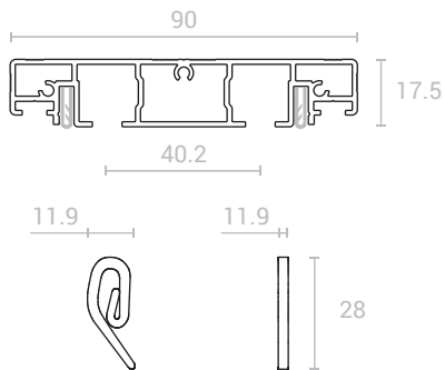
SLIM ROAD 02 Color: black, white Material: aluminum Compatible: textile, PVC
