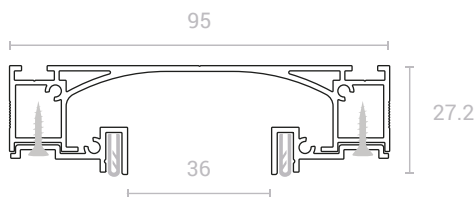
SLIM 35 Color: black, white, black-and-white Material: aluminum Compatible: textile, PVC
