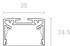
KBOX Length: 300/600/900 mm Color: black, white Material: aluminum
